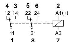
Connection diagram
