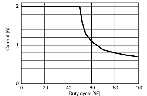
Fig. 2 Current vs. duty cycle
