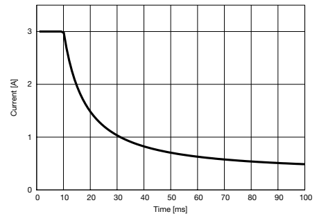
Fig.1 Inrush current
