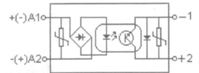
Fig. 1 CSS-DCP diagram
