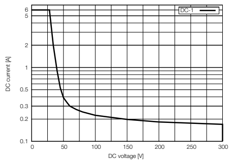
Fig. 2 DC load limit curve RINT 11, 21
