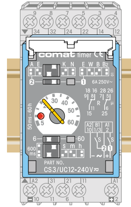
Connection diagram
